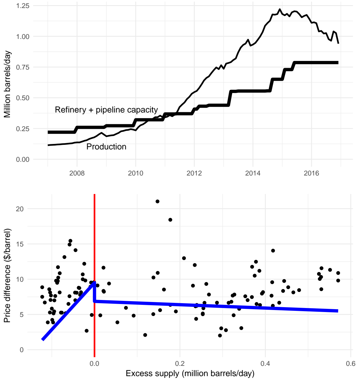
Figure A.1: Production, infrastructure, and price differentials for the Bakken region
